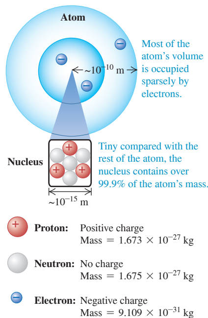
Figure 21.3 The structure of an atom. The particular atom depicted here is lithium (see Fig. 21.4a).
